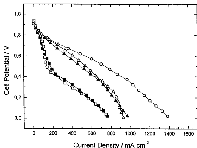
Fig. 4. H_2 + 100 ppm CO/O_2 polarization curves at 80^\circ\text{C} for a single membrane electrode assembly using (■) Pt_{0.5}-Ru_{0.5} (BM)-Mg and (▲) Pt_{0.5}-Ru_{0.5} ( Mg_4 ) at the anode. Polarization curves with (□) Pt Black, (○) Pt_{0.5}-Ru_{0.5} Black and (△) PtRuO_x at the anode are given for comparison.
