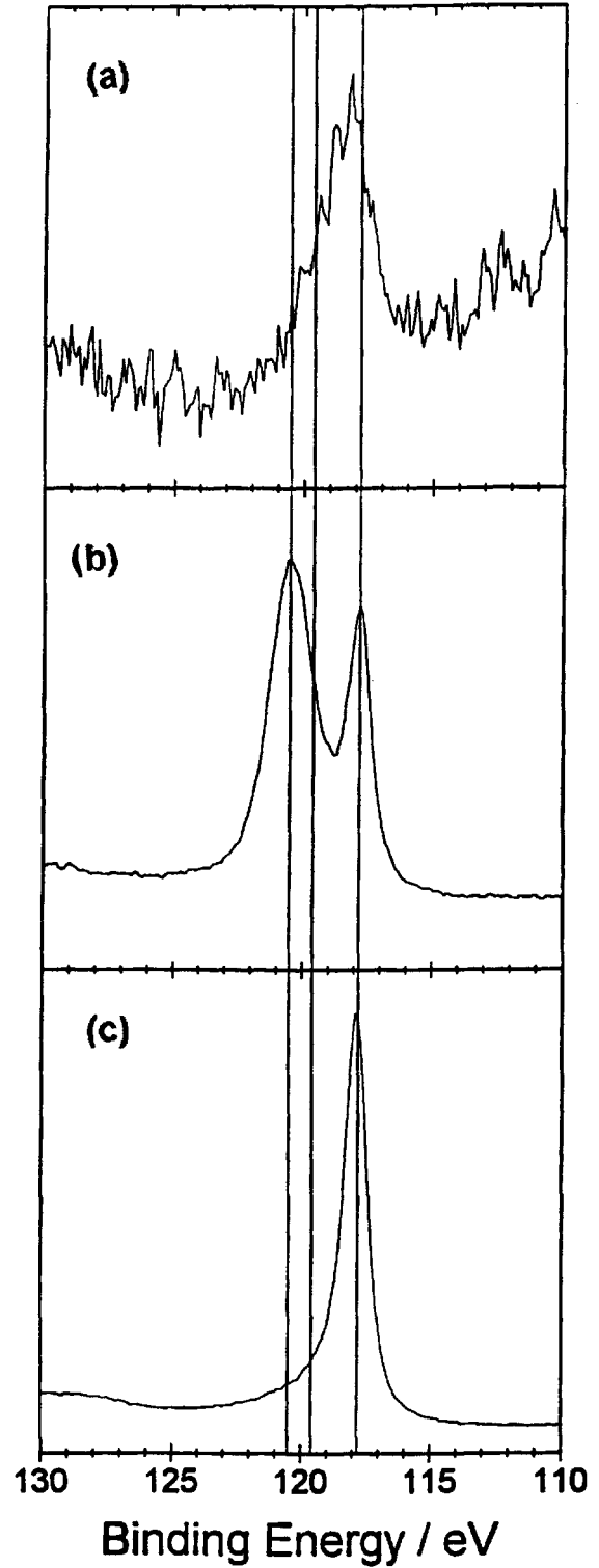
Fig. 10. XPS spectra at the Al 2s core level of (a) Pt 0.5 -Ru 0.5 (Al 4 ); (b) an Al film with its native oxidation layer and (c) an Al film after etching the oxidation layer. The vertical lines at 117.8, 119.6 and 120.5 eV are the binding energies for the Al 2s of Al, Al 2 O 3 , and oxidized metallic Al, respectively.
