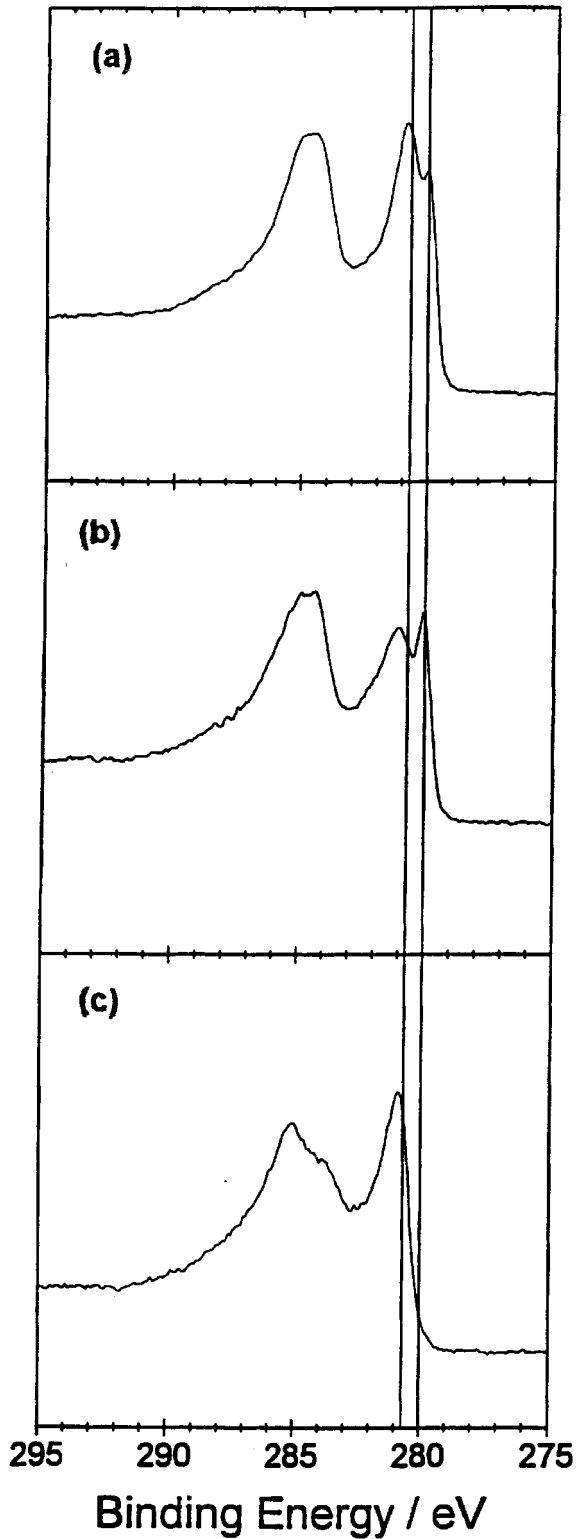
Fig. 9. XPS spectra at the Ru 3d core levels of (a) Pt 0.5 -Ru 0.5 Black; (b) Pt 0.5 -Ru 0.5 (Al 4 ); and (c) PtRuO x . The vertical lines at 280.0 and 280.7 eV are the binding energies reported for the 3d 5/2 peak of Ru and RuO 2 , respectively.
