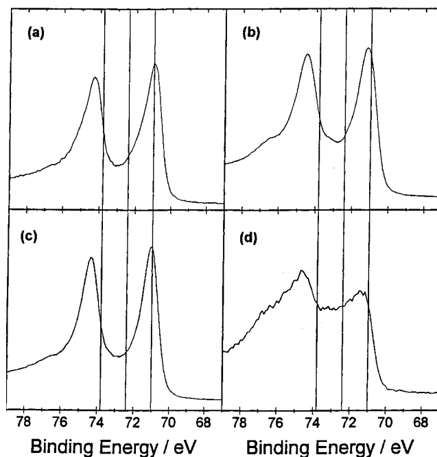
Fig. 8. XPS spectra at the Pt 4f core levels of (a) Pt Black; (b) \text{Pt}_{0.5}\text{-Ru}_{0.5} Black; (c) \text{Pt}_{0.5}\text{-Ru}_{0.5} ( \text{Al}_4 ); and (d) \text{PtRuO}_x . The vertical lines at 71.0, 72.4 and 73.8 eV are the binding energies reported for the 4f_{7/2} peaks of Pt, \text{Pt}(\text{OH})_2 and PtO, respectively.
